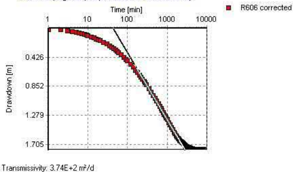
W601 Pumping test (Cooper-Jacob Time-Drawdown)
