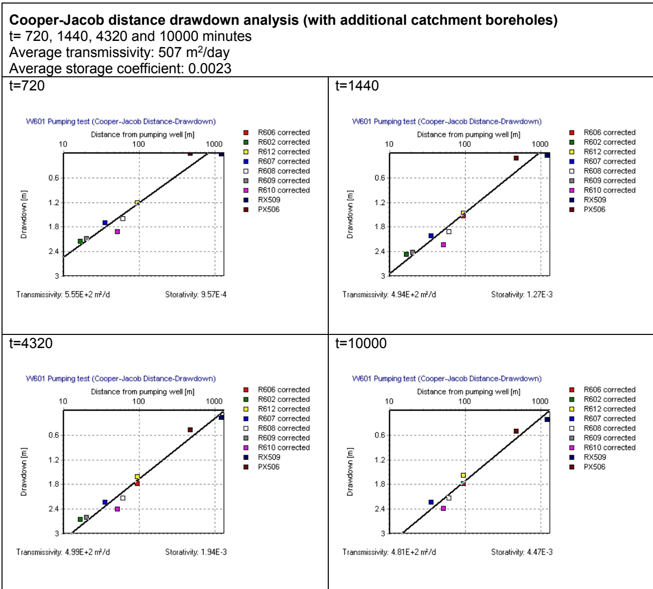
Figure 6.15 Cooper-Jacob distance drawdown analyses for W601 cluster, including catchment boreholes at 450 m and 1,200 m from the pumping well.
