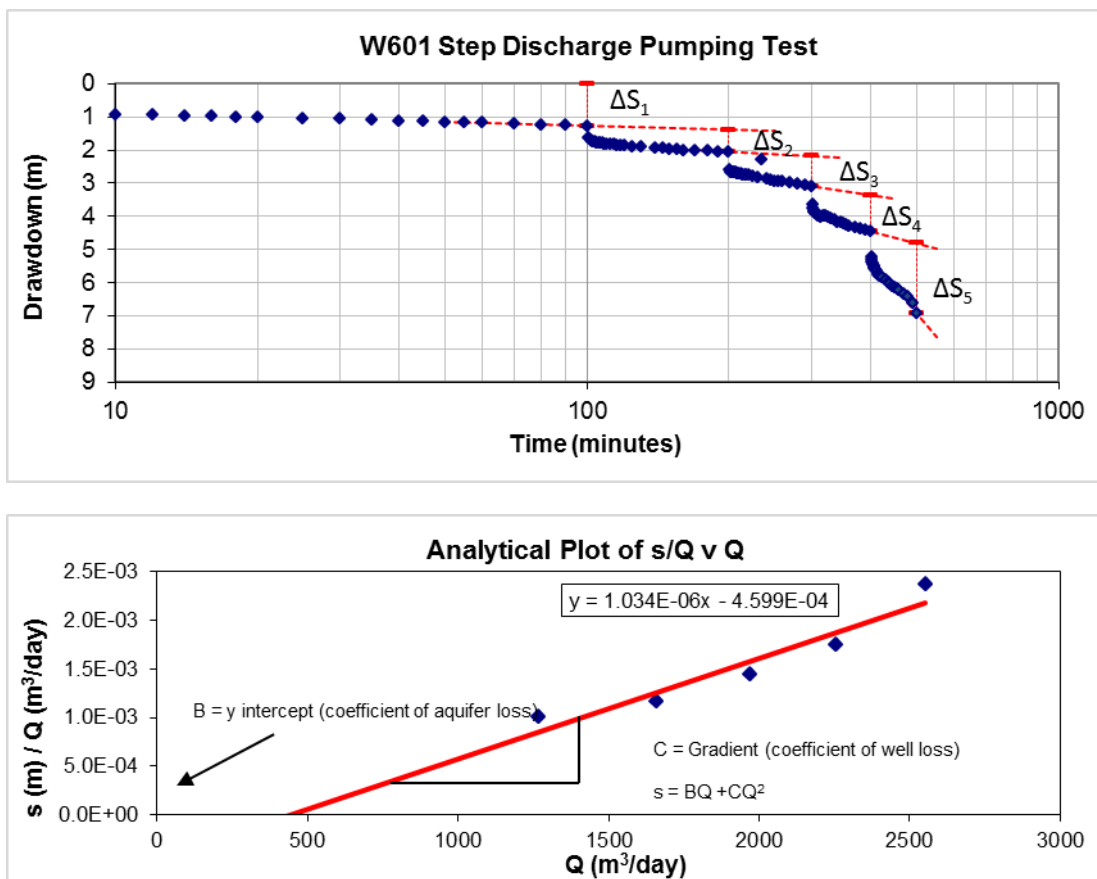
Figure 6.10 W601 Analysis charts
