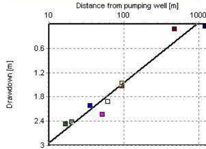
W601 Pumping test (Cooper-Jacob Distance-Drawdown)
