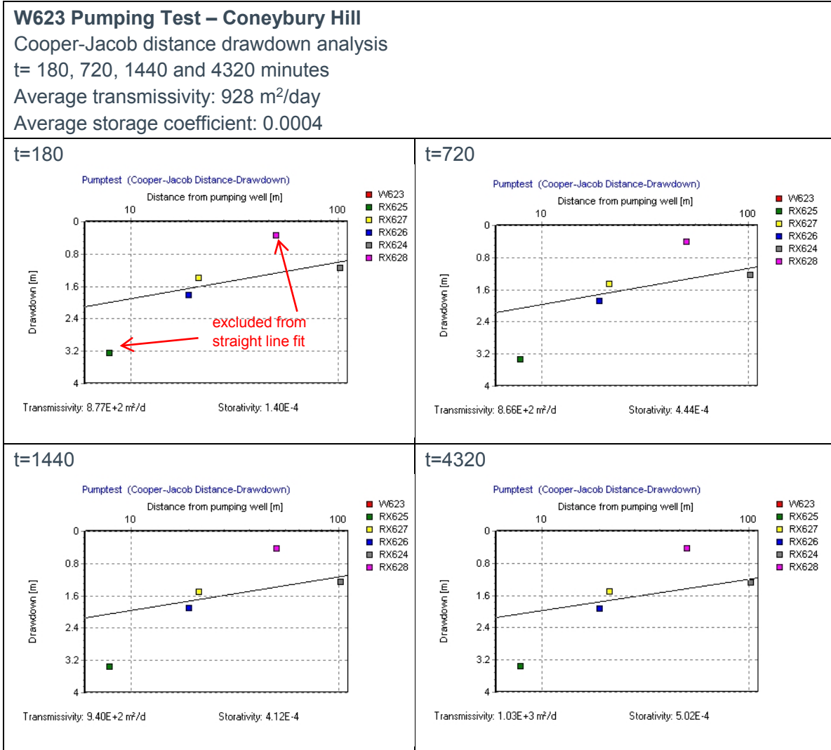
Figure 6.7 Distance drawdown analysis for W623
