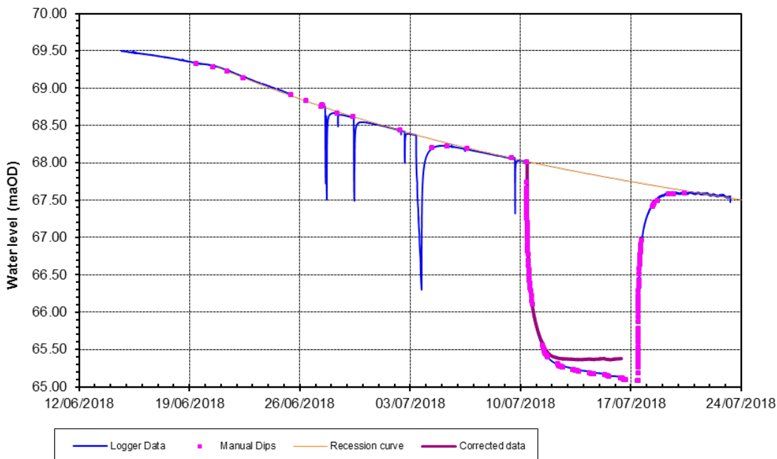
Figure 6.12 Recession curve defined using polynomial expression for R602
